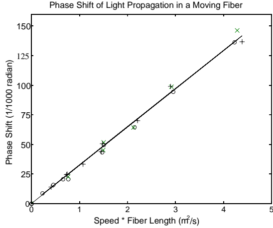
Fig. 3. FOC phase shifts versus products of fiber speeds and lengths. Symbol + is for the zero-area configuration, x for the figure-8 configuration, and o for the regular configuration. The straight line was found by a least square linear regression of all measurements.
