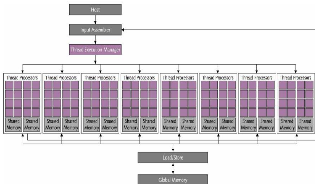
Figure 5. GPU Architecture.
