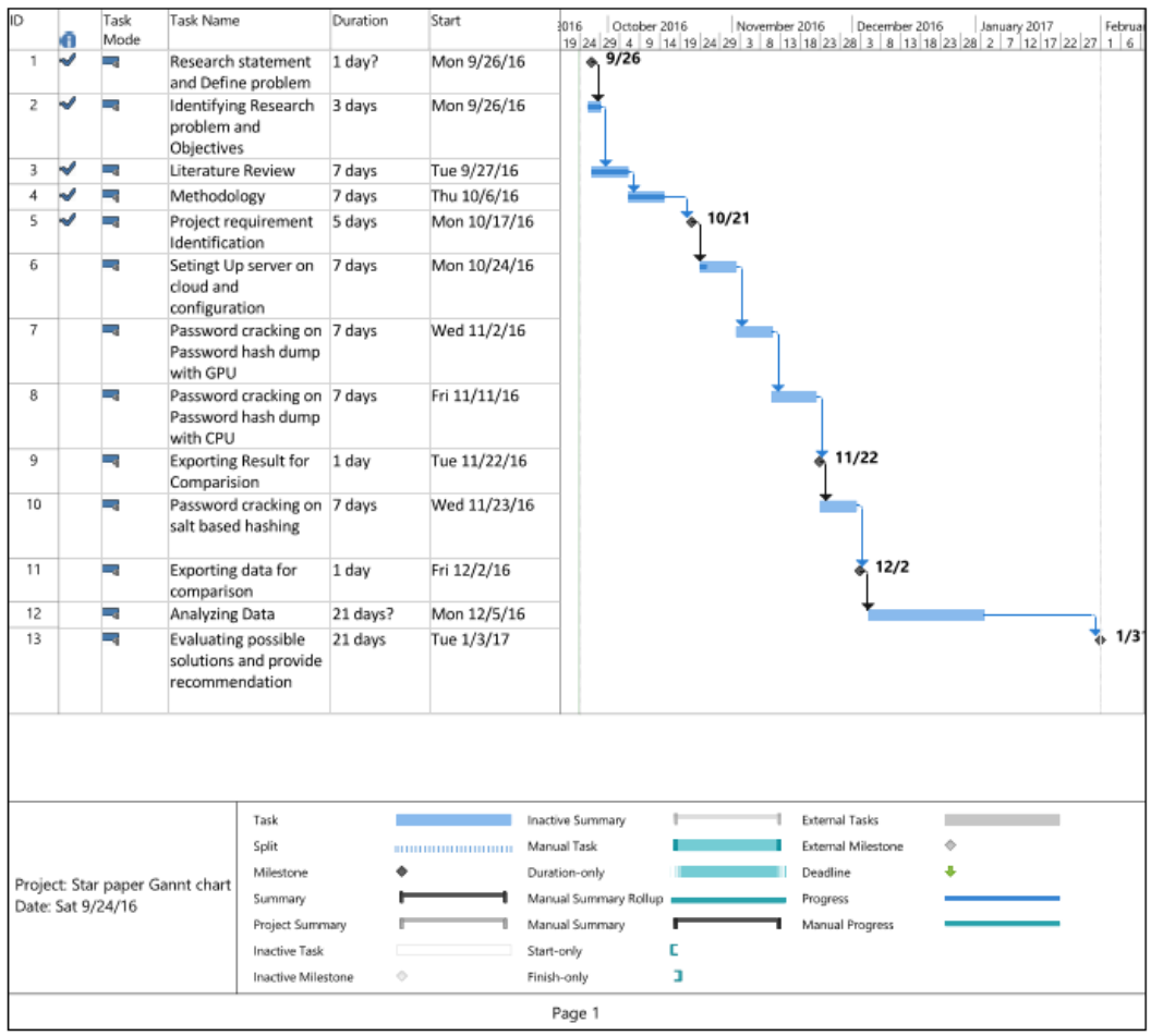
Figure 8. Project Timeline
