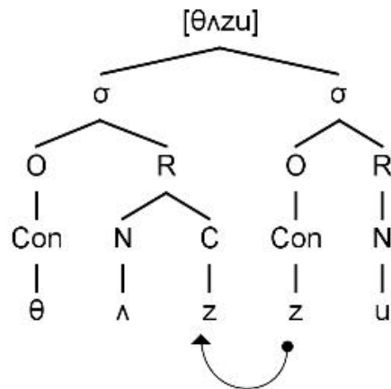
Figure 2: Syllable Diagram
