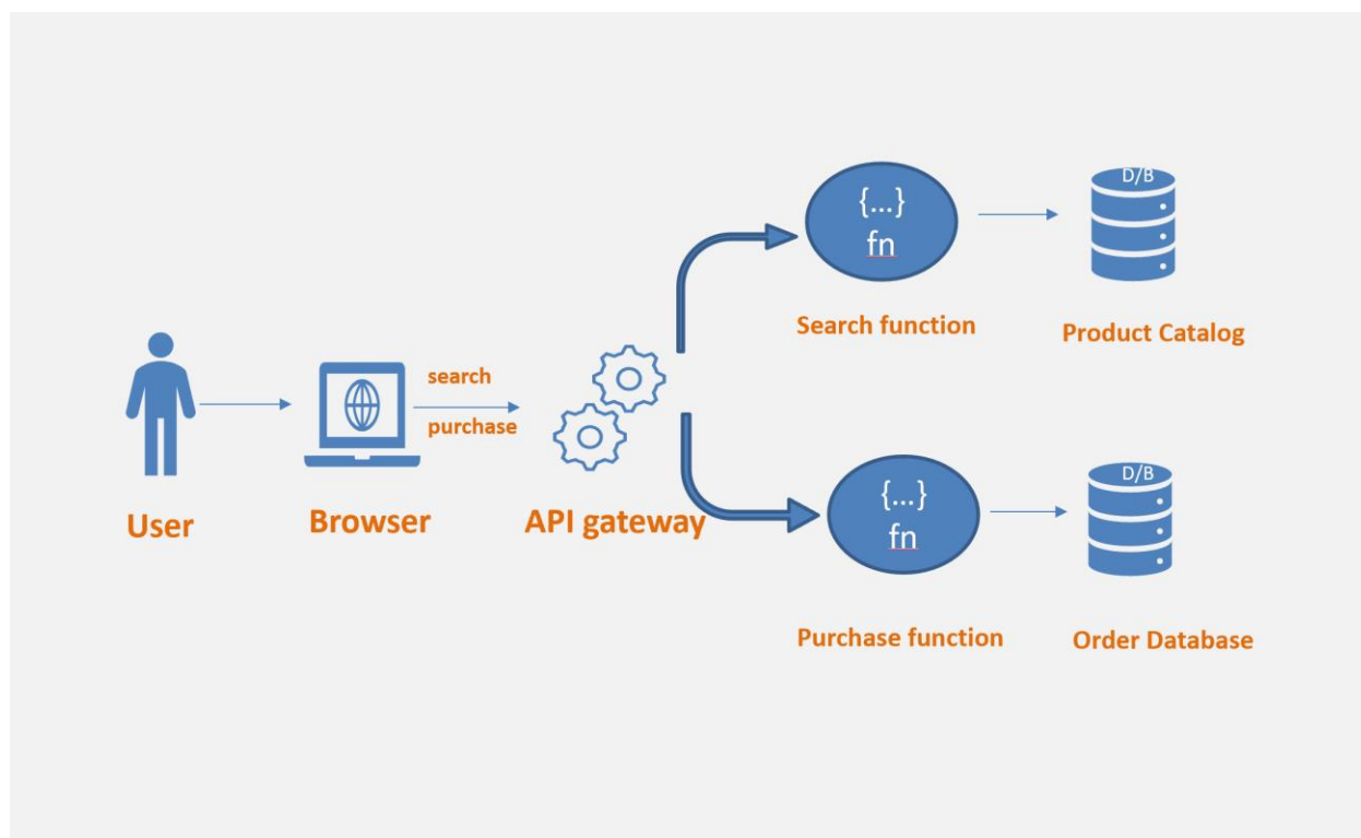
Serverless Architecture
